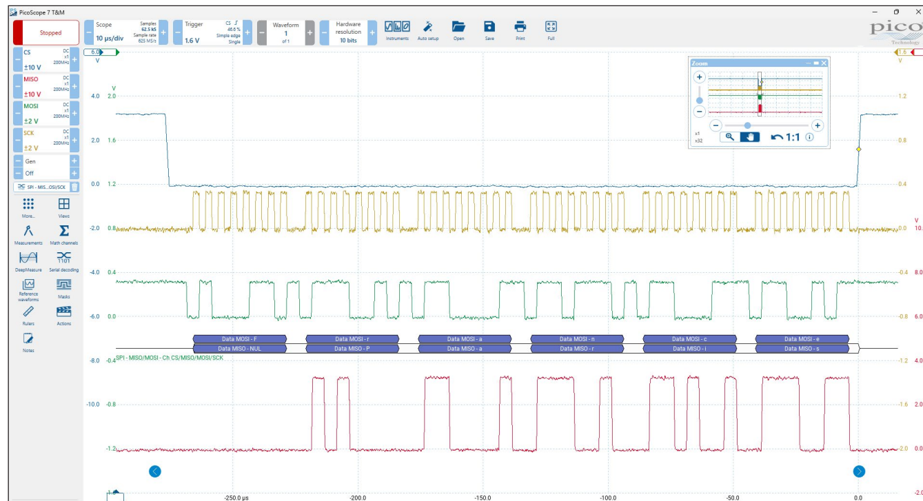
SPI interface
