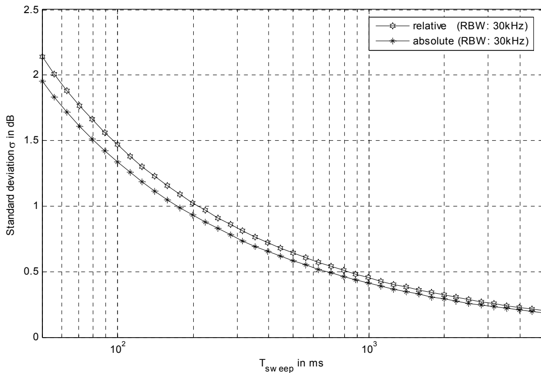
Standard deviation \sigma of spectrum emission mask measurement as a function of sweep time ( T_{\text{sweep}} )
