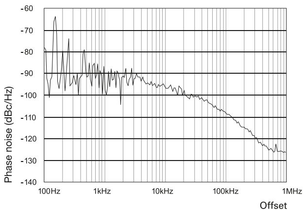
(Typical phase noise at 1 GHz)
