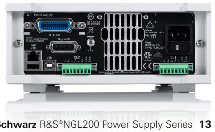
R&S®NGL202, rear view
