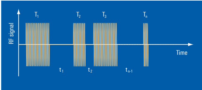
Pulse train.
