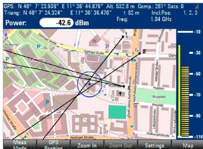
Display of map triangulation lines with R&S®FSH-K15.
