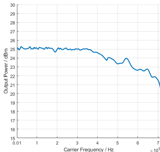
Measured maximum output power versus frequency with R&S®SMCVB-K31 option
