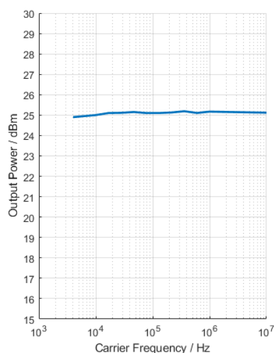
Measured maximum output power versus frequency with R&S®SMCVB-K31 option
