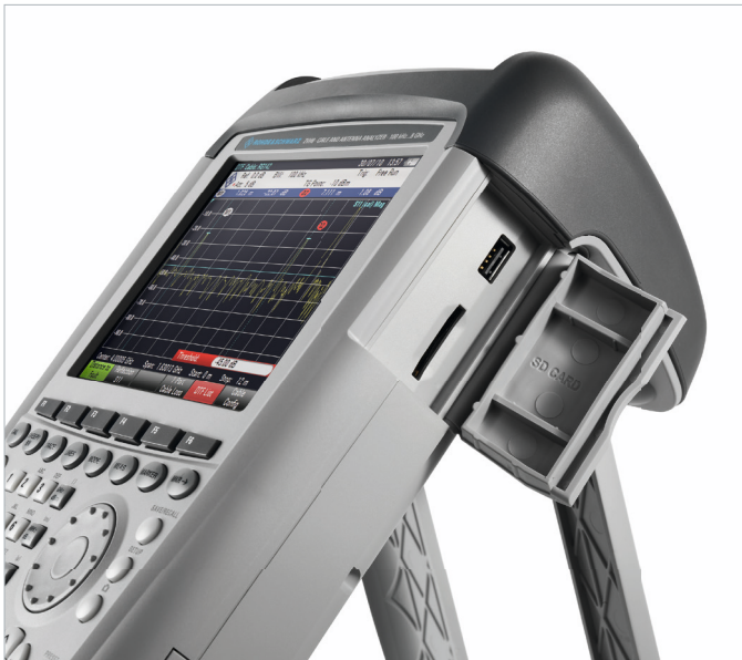
Additional connectors (e.g. for SD memory card and USB interface) are protected by hinged covers.
