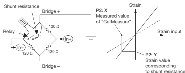
Gain correction using shunt CAL [gain correction on the negative (-) side]
