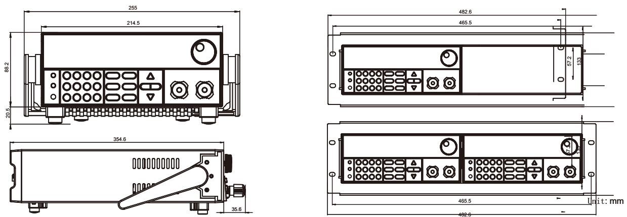
IT8811/12 Dimension figure 1/2 2U, 150 W~300 W
