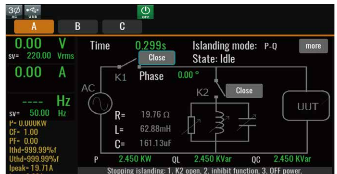
IT7900 Anti-islanding test
