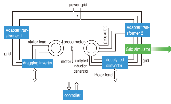
doubly fed converter test platform
